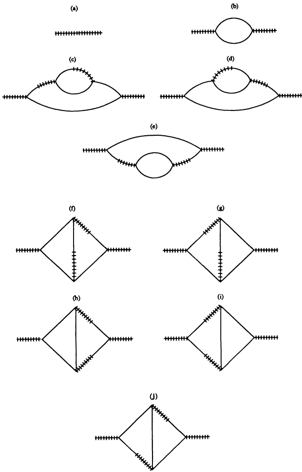
FIG. 7. Feynman diagrams for the dynamical perturbation expansion of \Gamma_{\bar{h}\bar{h}}(\mathbf{q}, \omega) to two-loop order.
